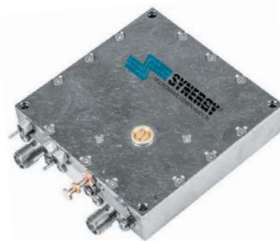
3. Phase-locked DROs from the KSFLD series offer low-noise signals from 6 to 15 GHz for system and test applications. (Courtesy of Synergy Microwave Corp.)
