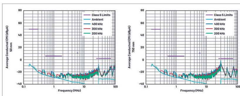
6. Current-probe CE comparison of switching frequencies.
