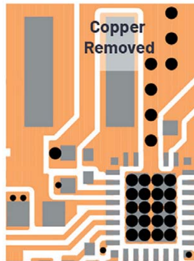
7. Switch-node cutoff area.
