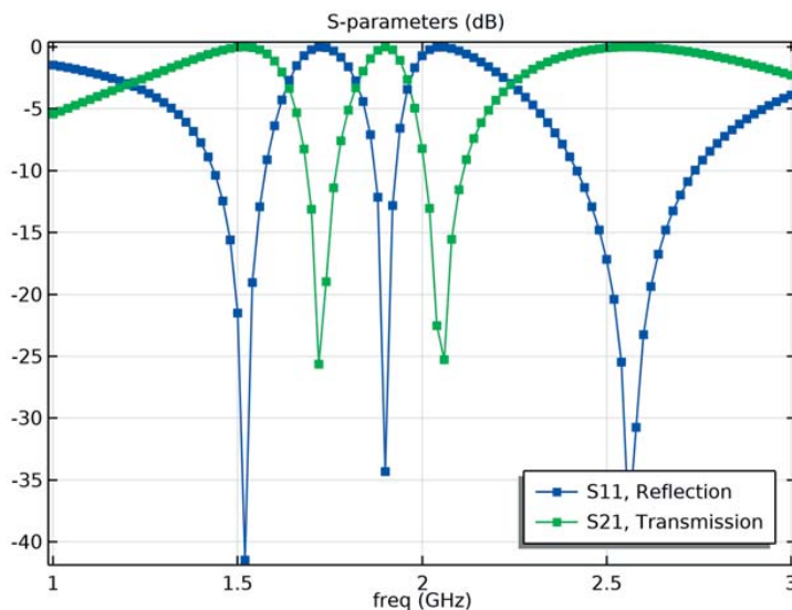
4. An S-parameter plot from 1 to 3 GHz shows the suggested frequency-selective surface's reflection and transmission characteristics.
