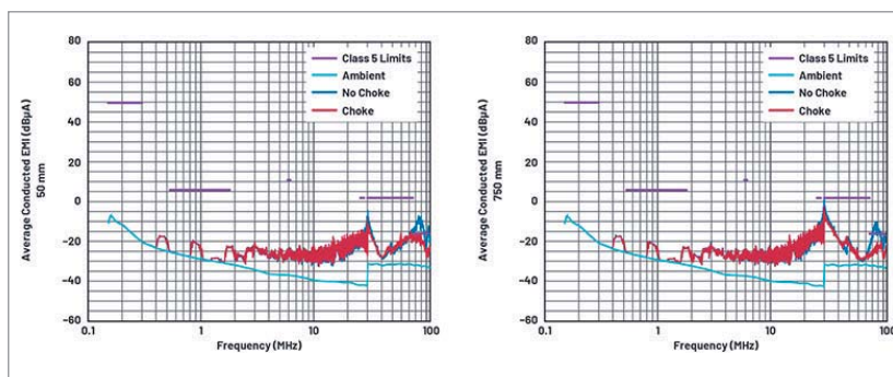
4. Current-probe CE shows that emissions are lower in the FM band when a common-mode choke is used.
